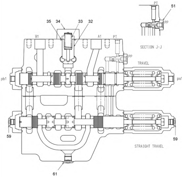
SECTION H-H
