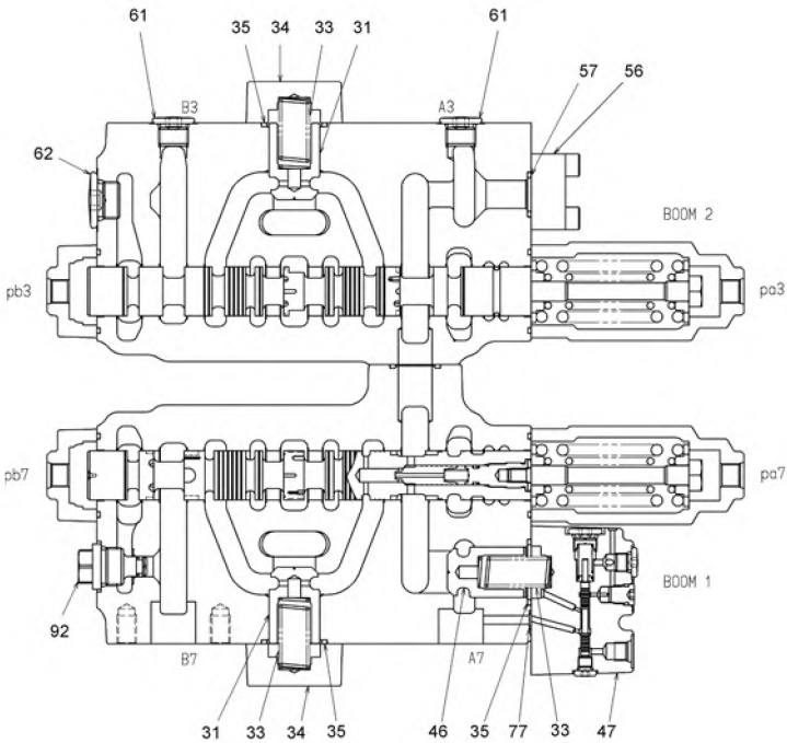
SECTION F-F
